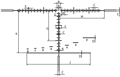
DMR8i RETICLE
