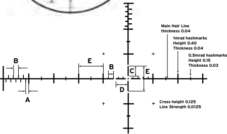
C2 RETICLE SUBTENSION
